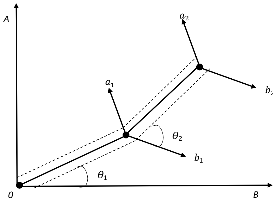
Figure 2: Two Link Arm Robot
